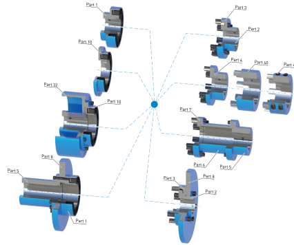
Modular principle of N-EUPEX types
